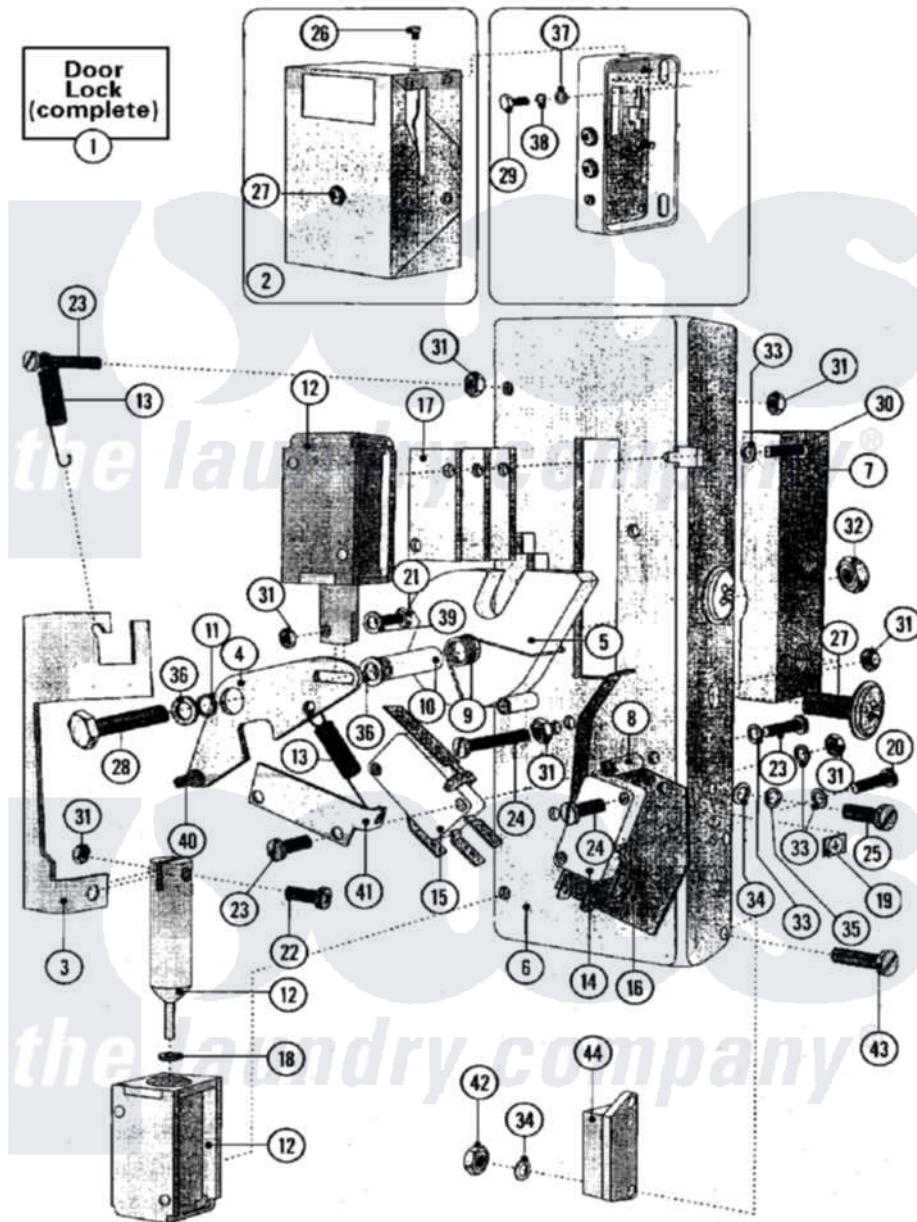
Maytag Residential Maytag MFS75PNAVS Washer Parts Parts Diagram 10 - DOOR LOCK Click on the part number to view part
