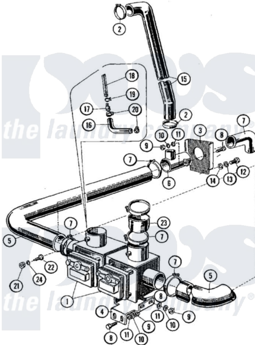
Maytag Residential Maytag MFX95PNAVS Washer Parts Parts Diagram 10 - DRAIN VALVE ASSEMBLY Click on the part number to view part
