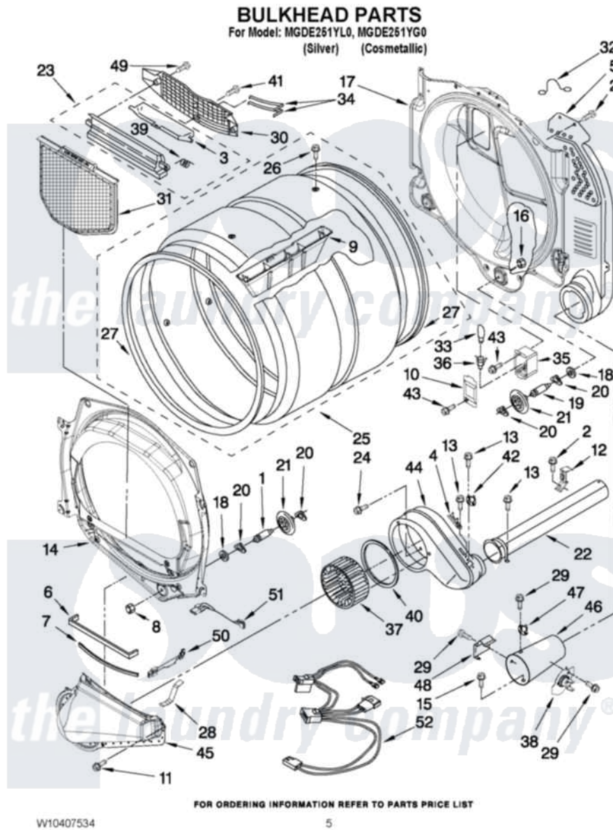
Maytag Residential Maytag MGDE251YL0 Dryer Parts Parts Diagram 03 - BULKHEAD PARTS Click on the part number to view part
