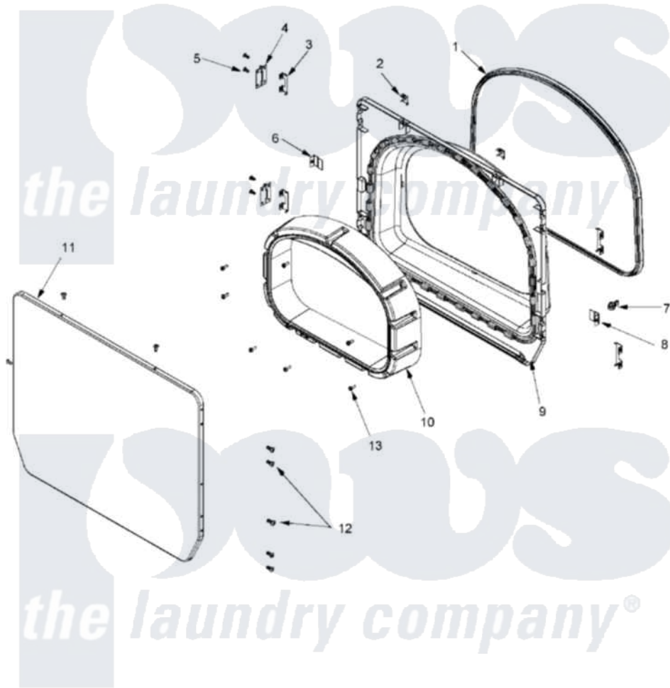
Maytag Residential Maytag MLE23PDHGW Dryer Parts Parts Diagram 05 - DOOR Click on the part number to view part
