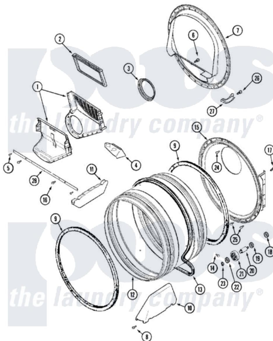
Maytag Residential Maytag MLE23PRAYW Dryer Parts Parts Diagram 07 - TUMBLER Click on the part number to view part
