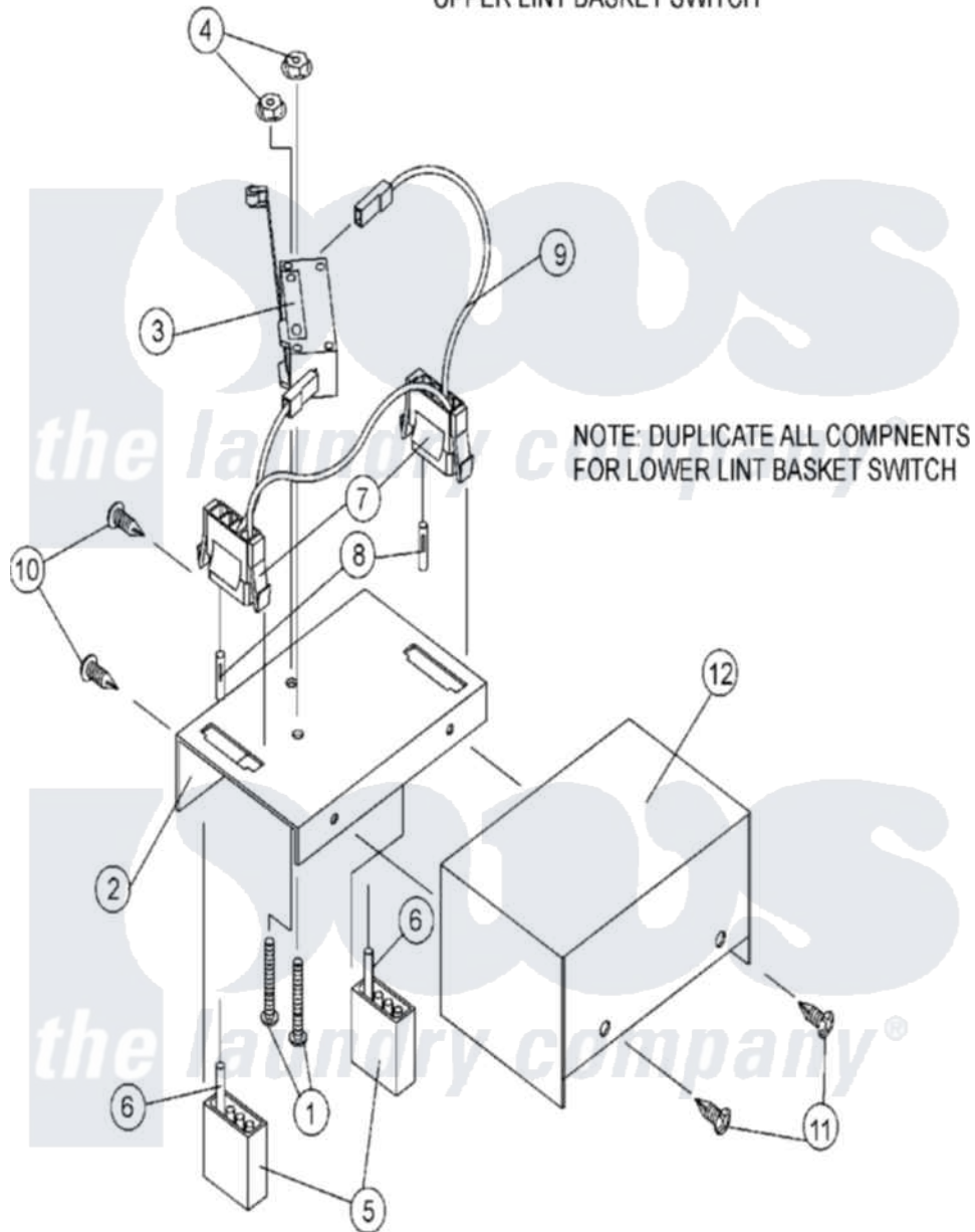
Maytag Residential Maytag MLG31PCAWS Dryer Parts Parts Diagram 15 - LINT DRAWER SWITCH ASSEMBLY
