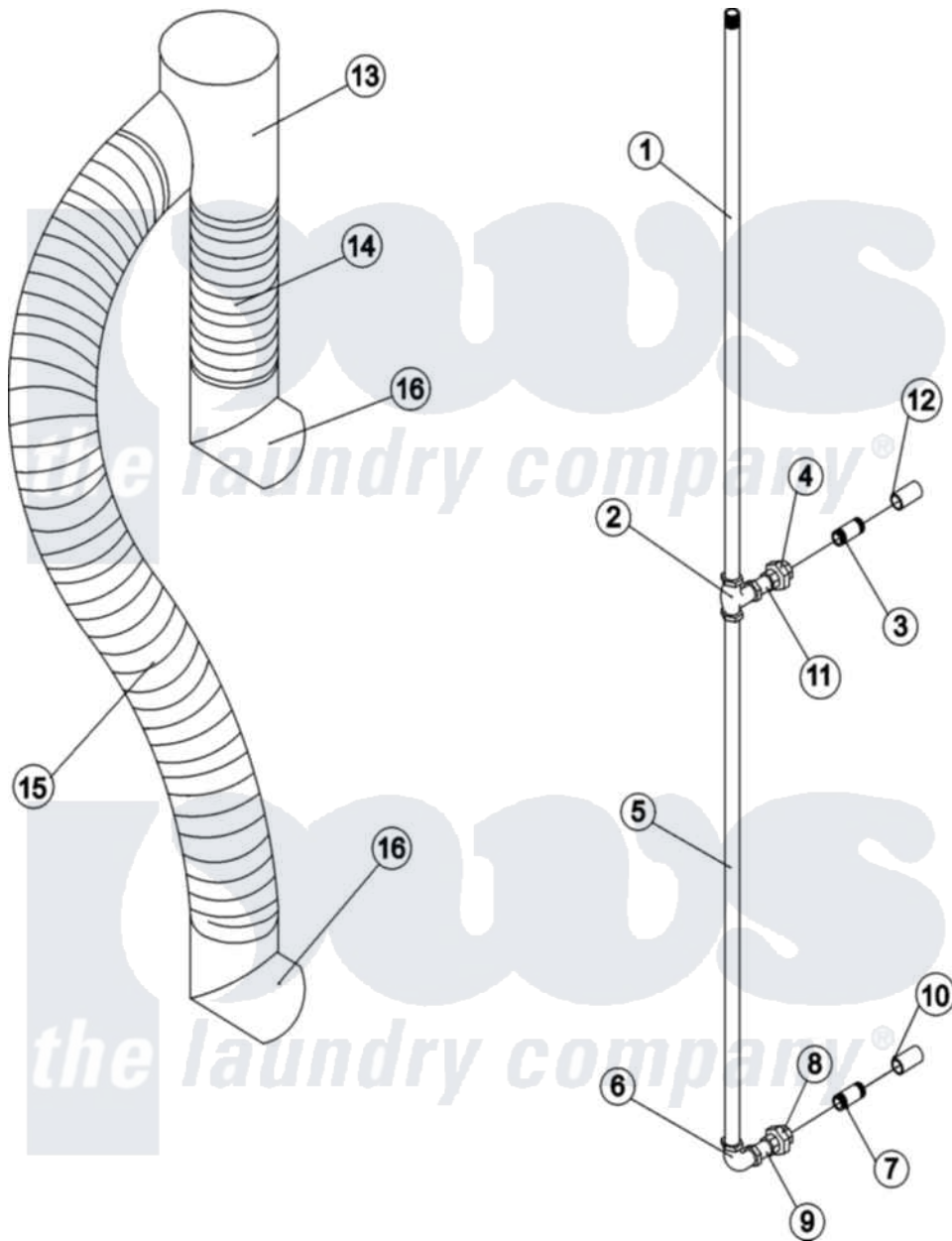
Maytag Residential Maytag MLG31PCAWS Dryer Parts Parts Diagram 21 - OPTIONAL PIPING & DUCTING KITS
