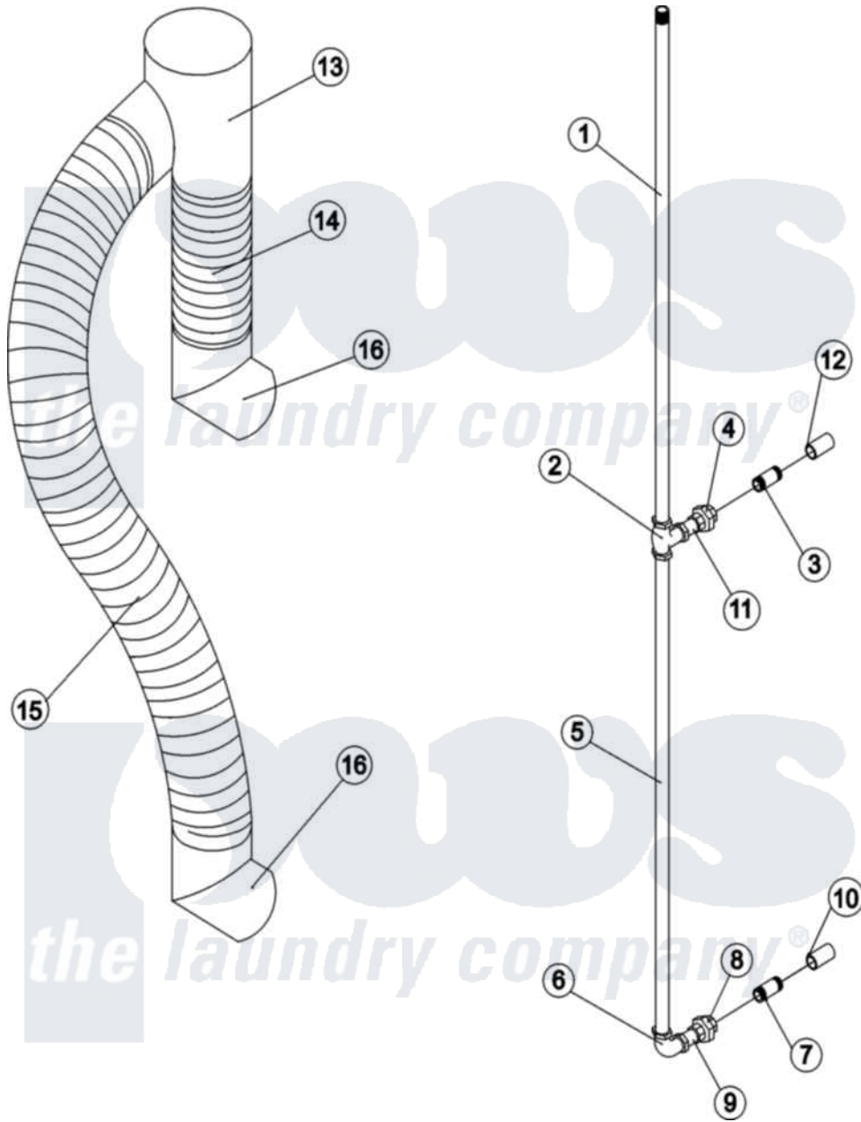
Maytag Residential Maytag MLG31PCAWW Dryer Parts Parts Diagram 21 - OPTIONAL PIPING & DUCTING KITS
