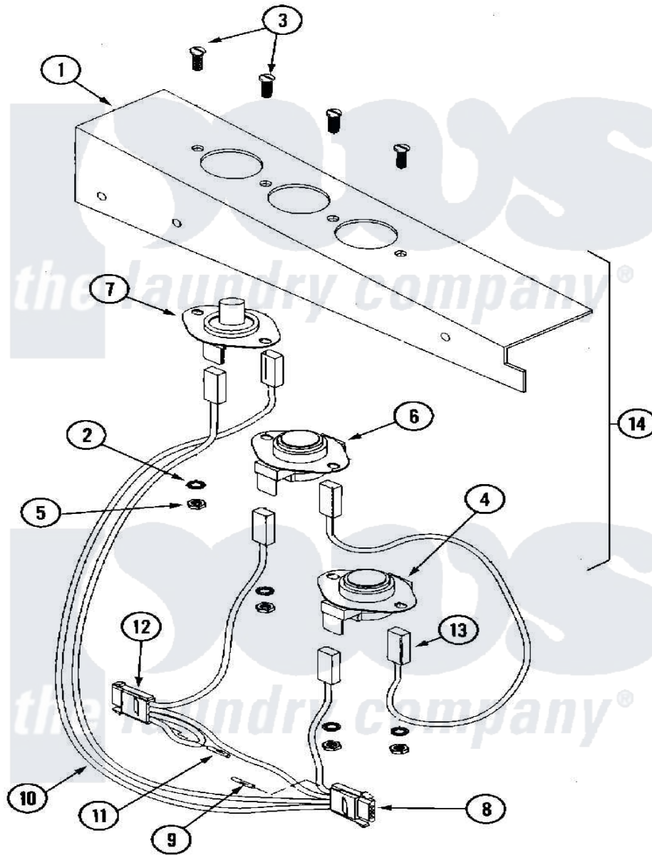
Maytag Residential Maytag MLG32PDAWA Dryer Parts Parts Diagram 08 - TEMP. SENSOR BRKT. ASSEMBLY (MLG32PDAWx)
