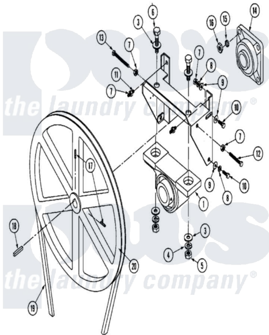
Maytag Residential Maytag MLG32PDAWA Dryer Parts Parts Diagram 25 - TUMBLER BEARING ASSEMBLY (MLG32PDBWx)
