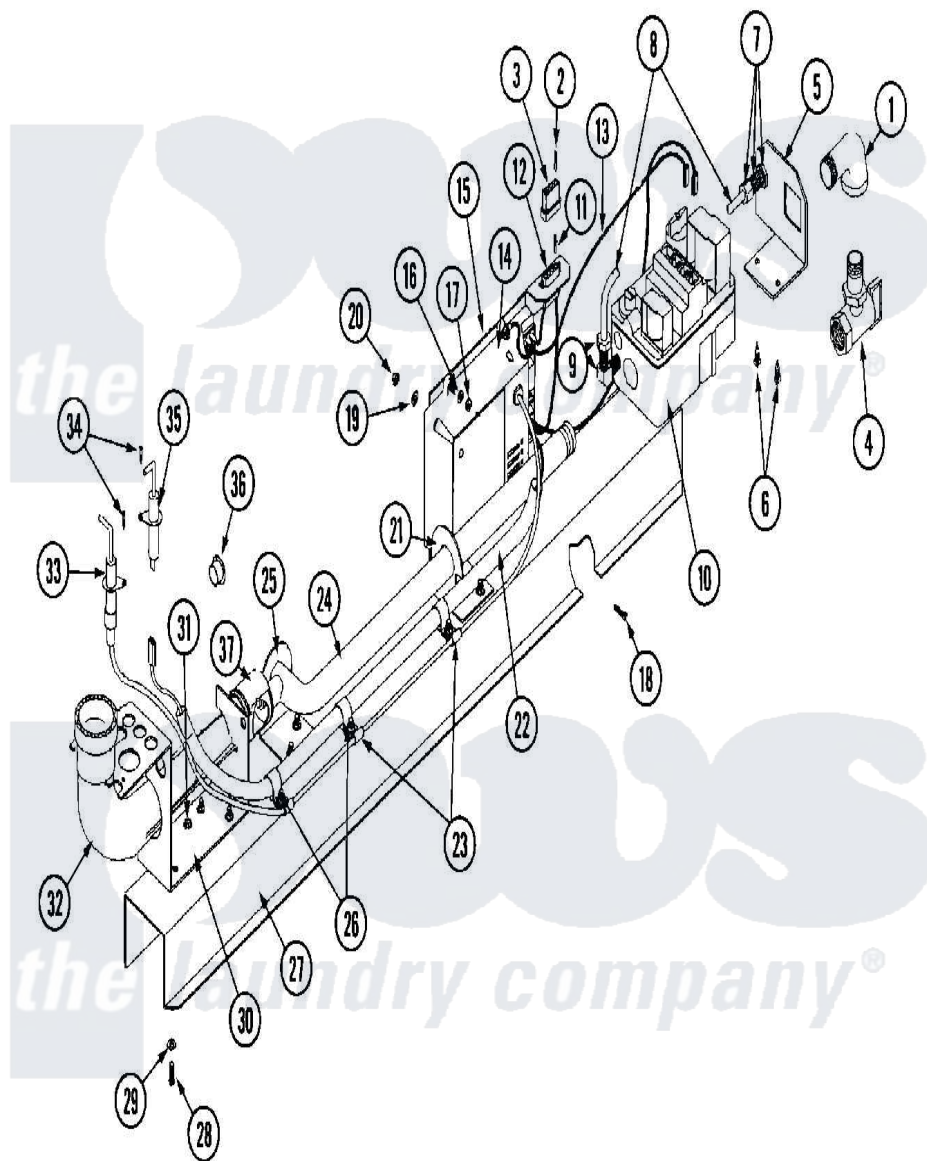
Maytag Residential Maytag MLG32PDBWW Dryer Parts Parts Diagram 11 - GAS VALVE ASSEMBLY (PRIOR TO YW SERIALNo.)
