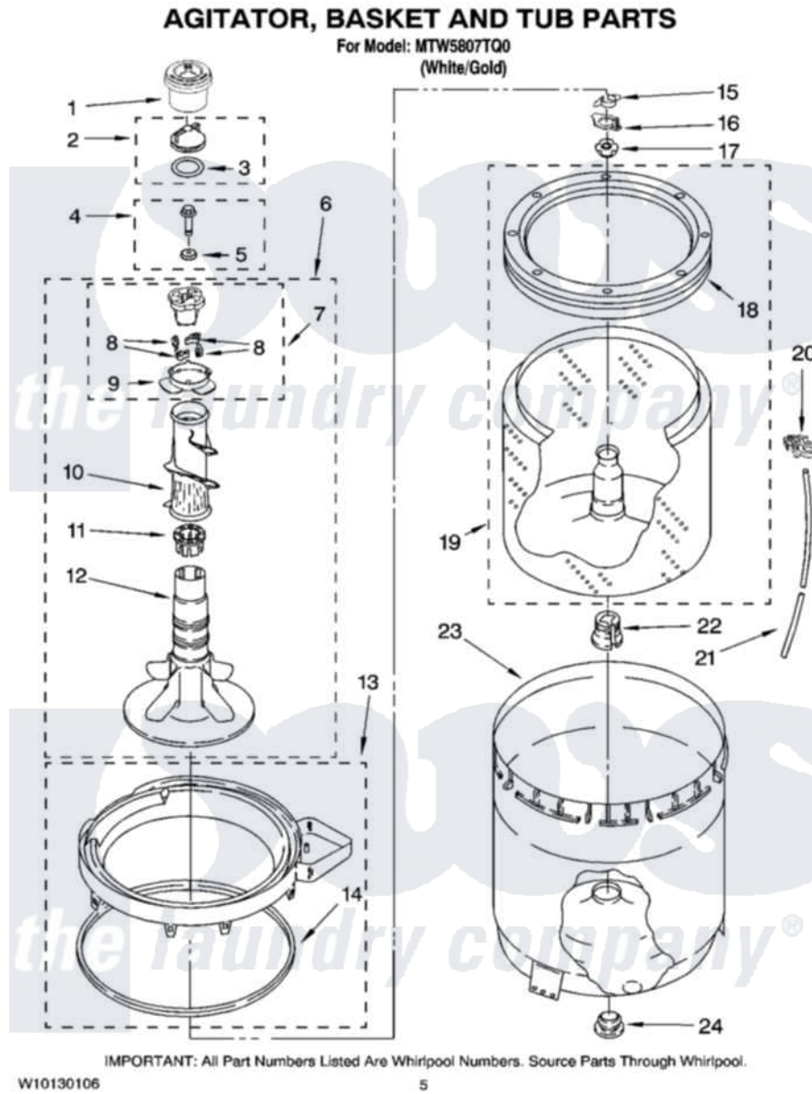
Maytag Residential Maytag MTW5807TQ0 Washer Parts Diagram 03 - AGITATOR, BASKET AND TUB PARTS
