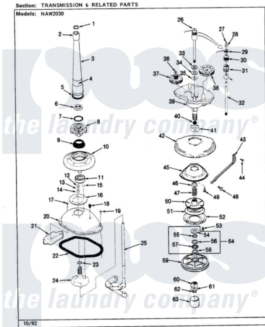
Maytag Residential Maytag NAW2030A Washer Parts Diagram 07 - TRANSMISSION & RELATED PARTS (REV. F-K)
