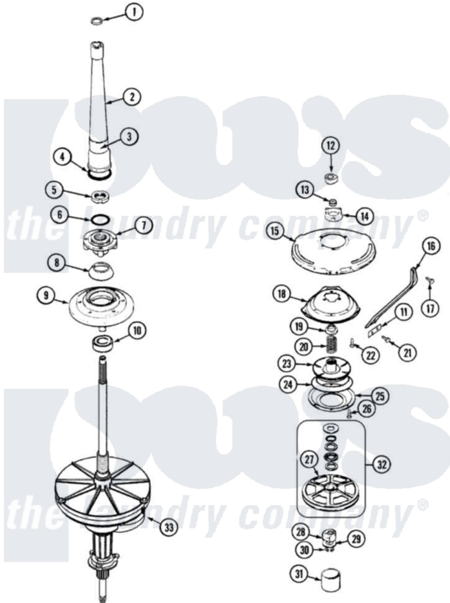
Maytag Residential Maytag PAV2000AAW Washer Parts Parts Diagram 05 - TRANSMISSION, DUAL DRIVE Click on the part number to view part
