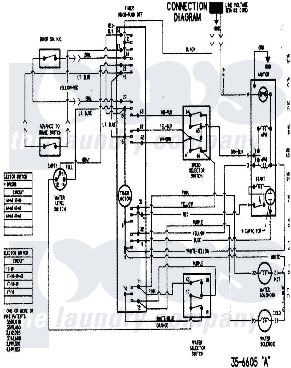
Maytag Residential Maytag PAV3240AWW Washer Parts Diagram 11 - WIRING INFORMATION (SERIES 20)
