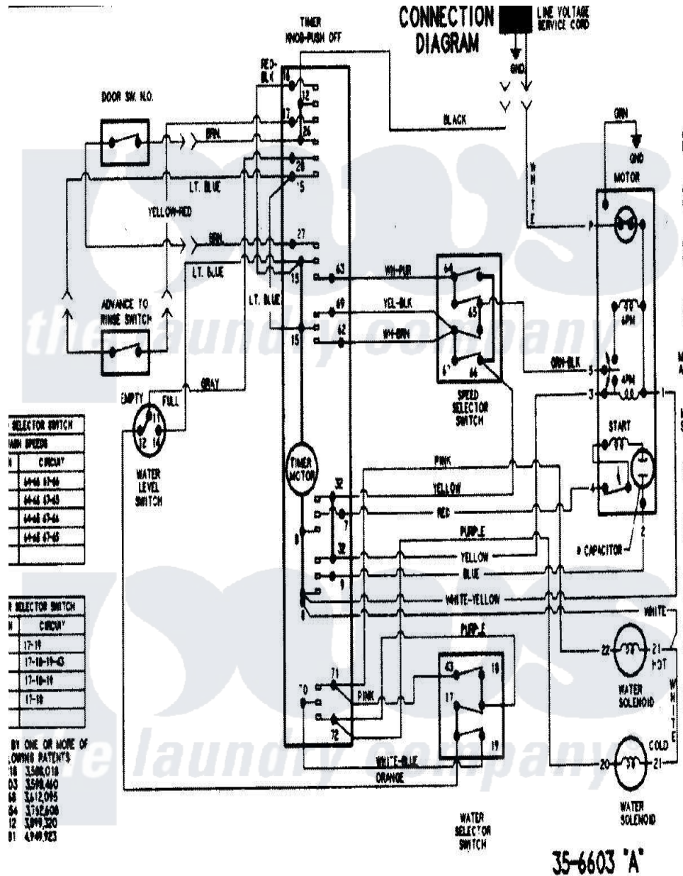
Maytag Residential Maytag PAV3300AWW Washer Parts Diagram 11 - WIRING INFORMATION (SERIES 20)
