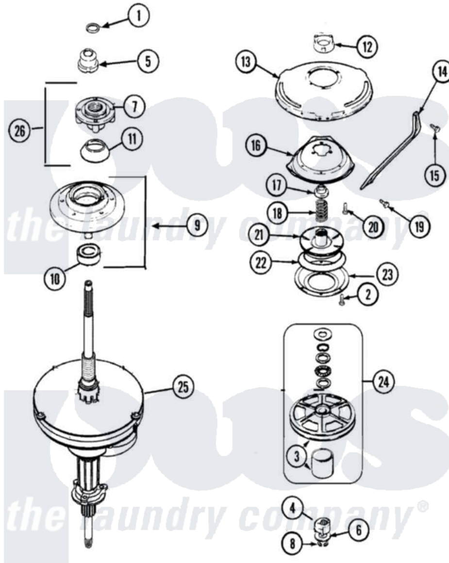
Maytag Residential Maytag PAV4960AWW Washer Parts Parts Diagram 08 - TRANSMISSION Click on the part number to view part
