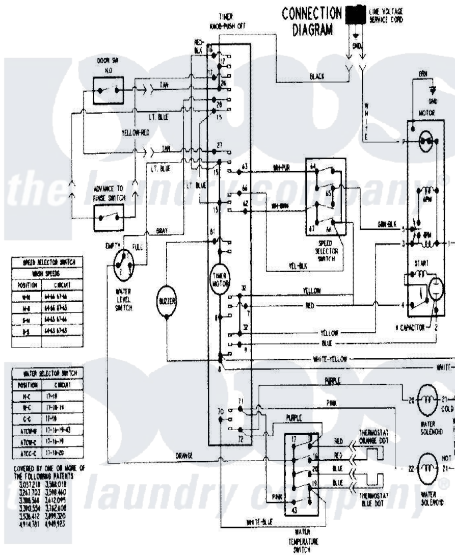
Maytag Residential Maytag PAV5057AWW Washer Parts Parts Diagram 08 - WIRING INFORMATION Click on the part number to view part
