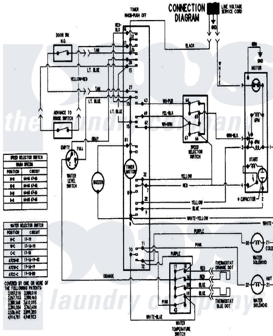
Maytag Residential Maytag PAV5157AWW Washer Parts Parts Diagram 11 - WIRING INFORMATION Click on the part number to view part
