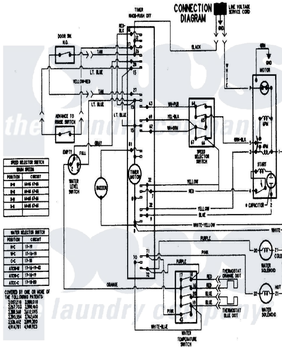
Maytag Residential Maytag PAV5158AWW Washer Parts Parts Diagram 11 - WIRING INFORMATION Click on the part number to view part
