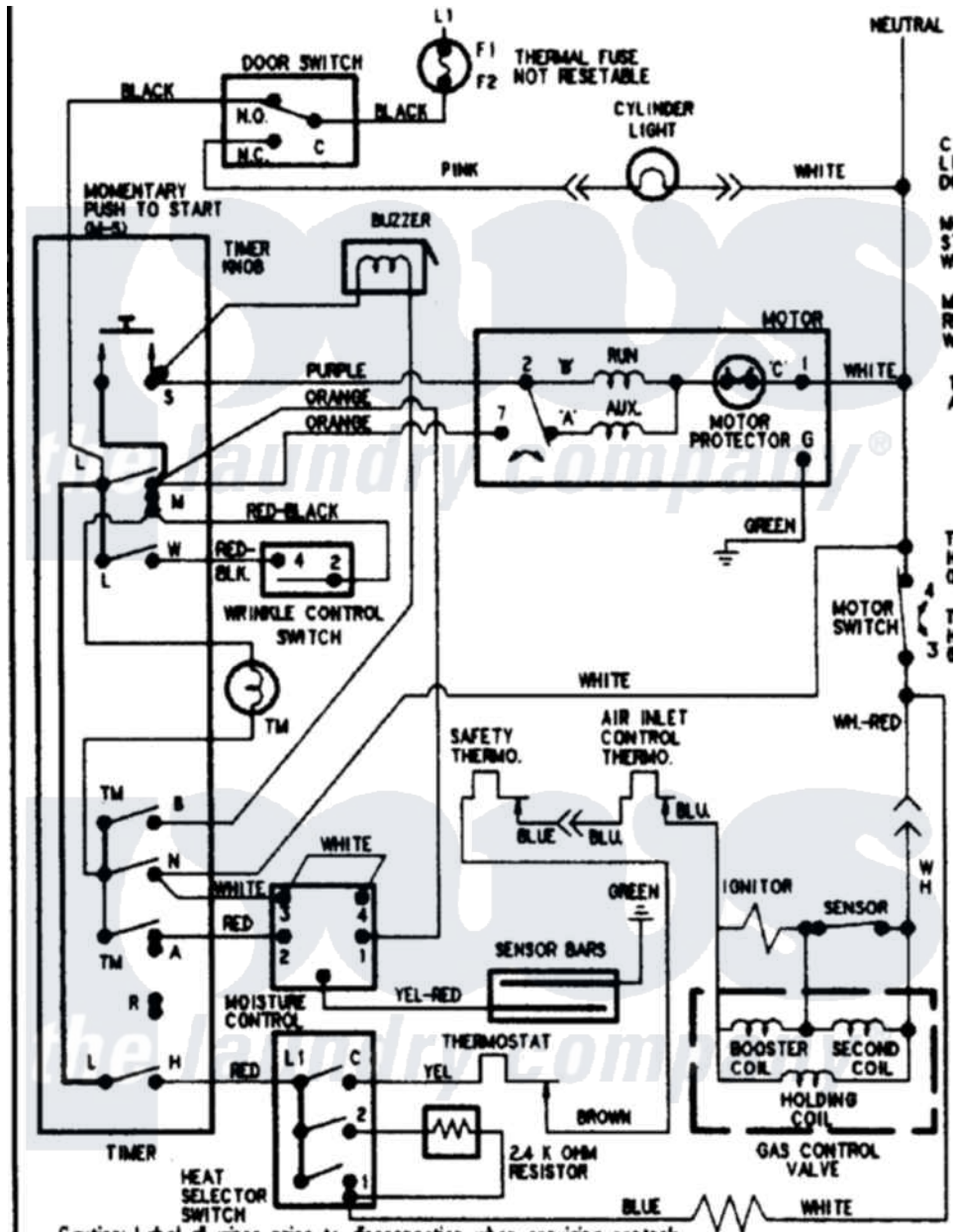
Maytag Residential Maytag PYG4500AWQ Dryer Parts Diagram 08 - WIRING INFORMATION Click on the part number to view part
