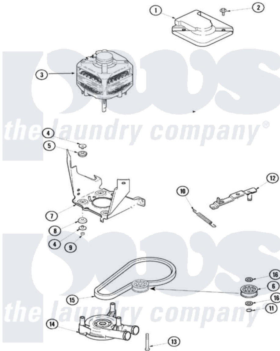
Maytag Residential Maytag SAV365AAWW Washer Parts Parts Diagram 04 - MOTOR, PUMP AND IDLER ASSEMBLY
