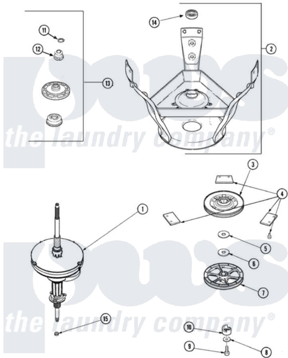
Maytag Residential Maytag SAV505DAWW Washer Parts Parts Diagram 07 - TRANSMISSION & BRAKE Click on the part number to view part
