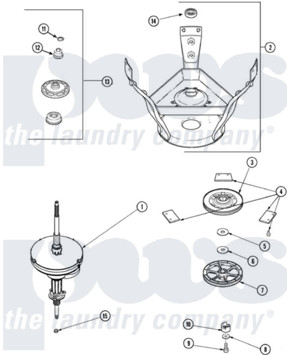
Maytag Residential Maytag SAV5701AWW Washer Parts Parts Diagram 07 - TRANSMISSION & BRAKE Click on the part number to view part
