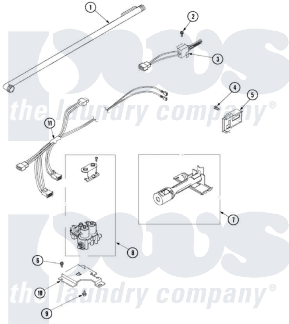
Maytag Residential Maytag SDG505DAWW Dryer Parts Parts Diagram 05 - GAS VALVE & IGNITER Click on the part number to view part
