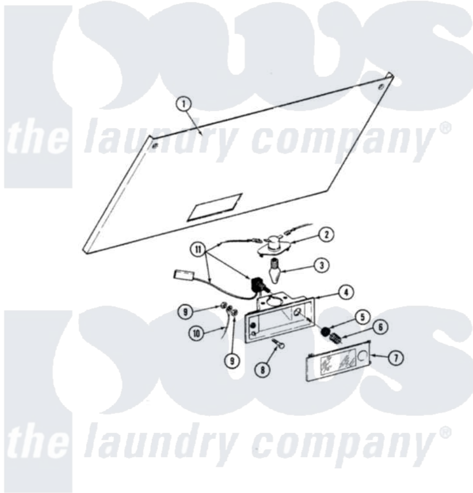
Maytag Residential Maytag SE9900 Stacked Washer and Dryer Parts Parts Diagram 01 - ACCESS PANEL & TUB LIGHT
