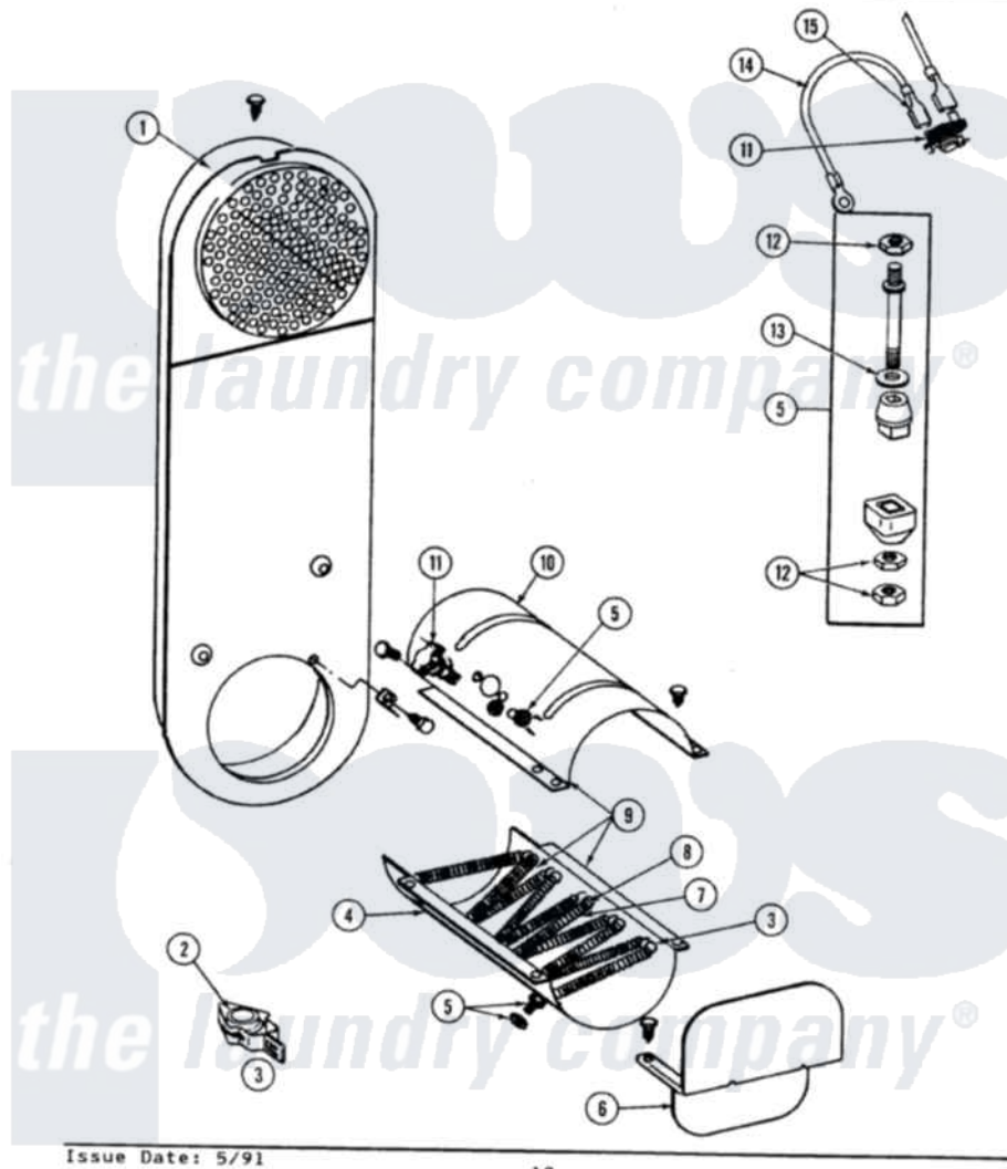
Maytag Residential Maytag SG1000 Stacked Washer and Dryer Parts Parts Diagram 10 - INLET DUCT & HEATER ASSEMBLY (SE1000)
