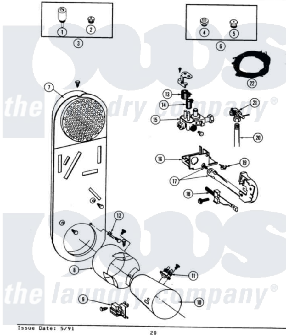
Maytag Residential Maytag SG1000 Stacked Washer and Dryer Parts Parts Diagram 11 - INLET DUCT & HEATER ASSEMBLY (SG1000)
