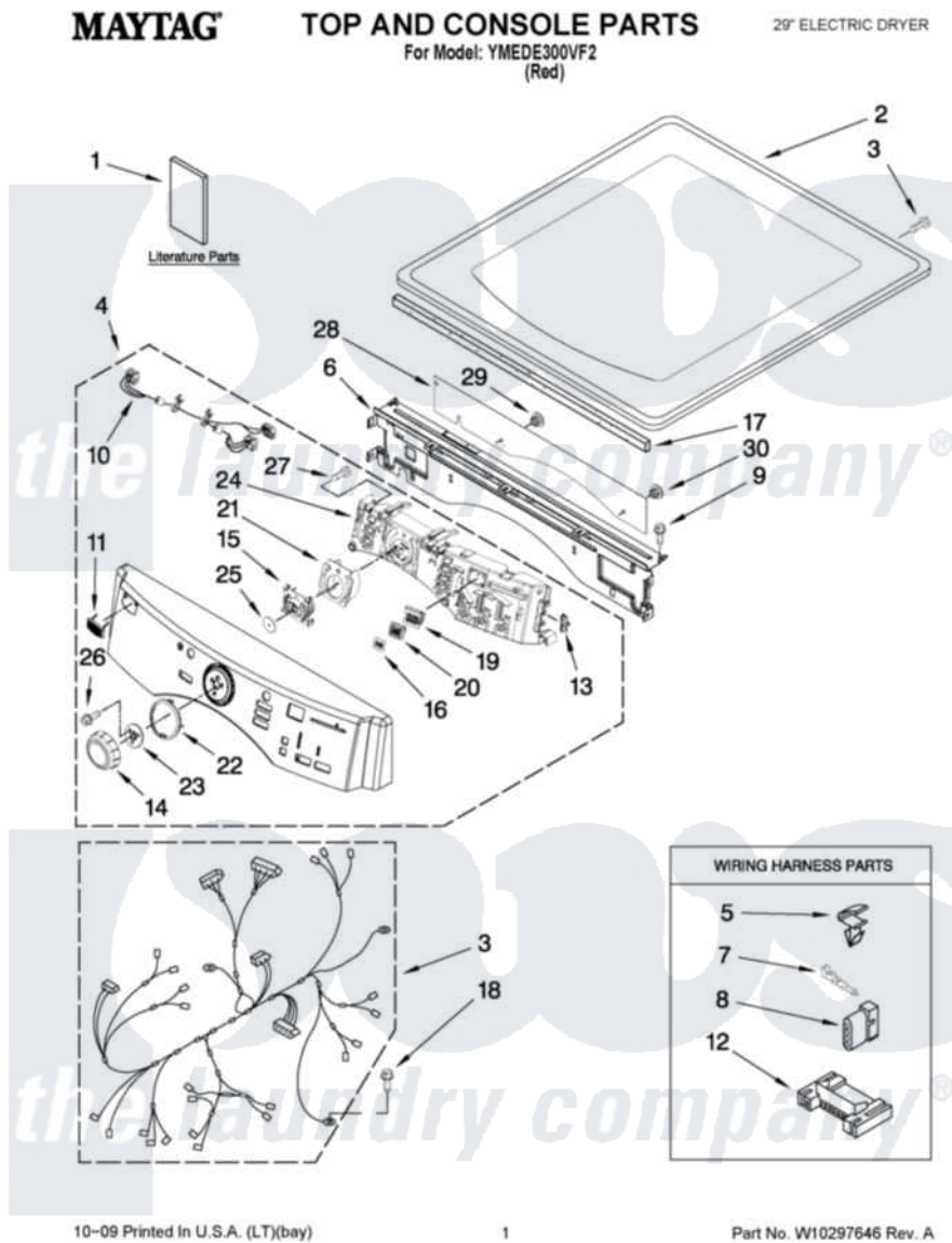
Maytag Residential Maytag YMEDE300VF2 Dryer Parts Parts Diagram 01 - TOP AND CONSOLE PARTS Click on the part number to view part
