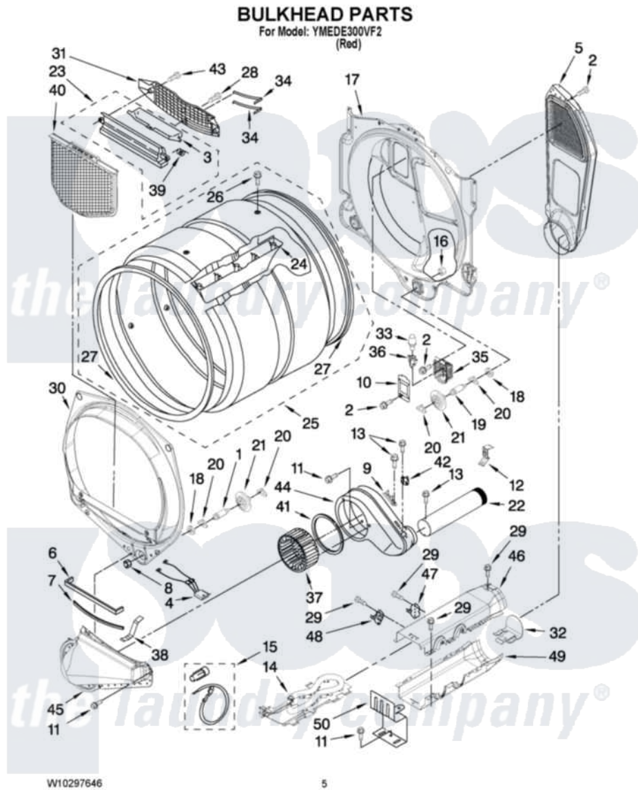
Maytag Residential Maytag YMEDE300VF2 Dryer Parts Parts Diagram 03 - BULKHEAD PARTS Click on the part number to view part
