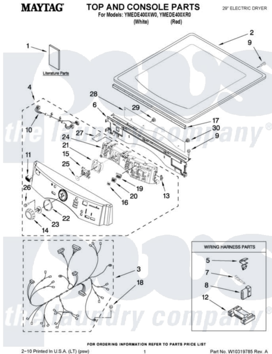
Maytag Residential Maytag YMEDE400XR0 Dryer Parts Parts Diagram 01 - TOP AND CONSOLE PARTS Click on the part number to view part
