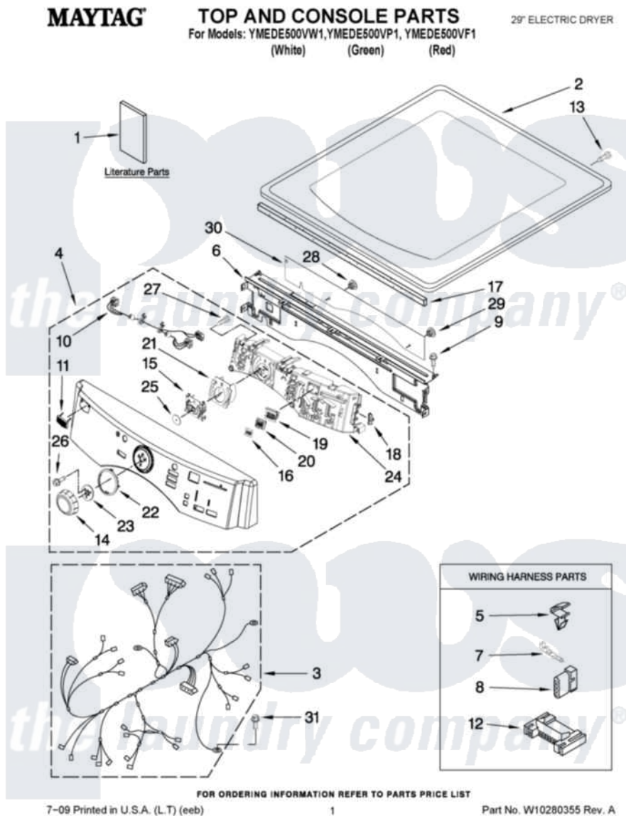
Maytag Residential Maytag YMEDE500VF1 Dryer Parts Parts Diagram 01 - TOP AND CONSOLE PARTS Click on the part number to view part
