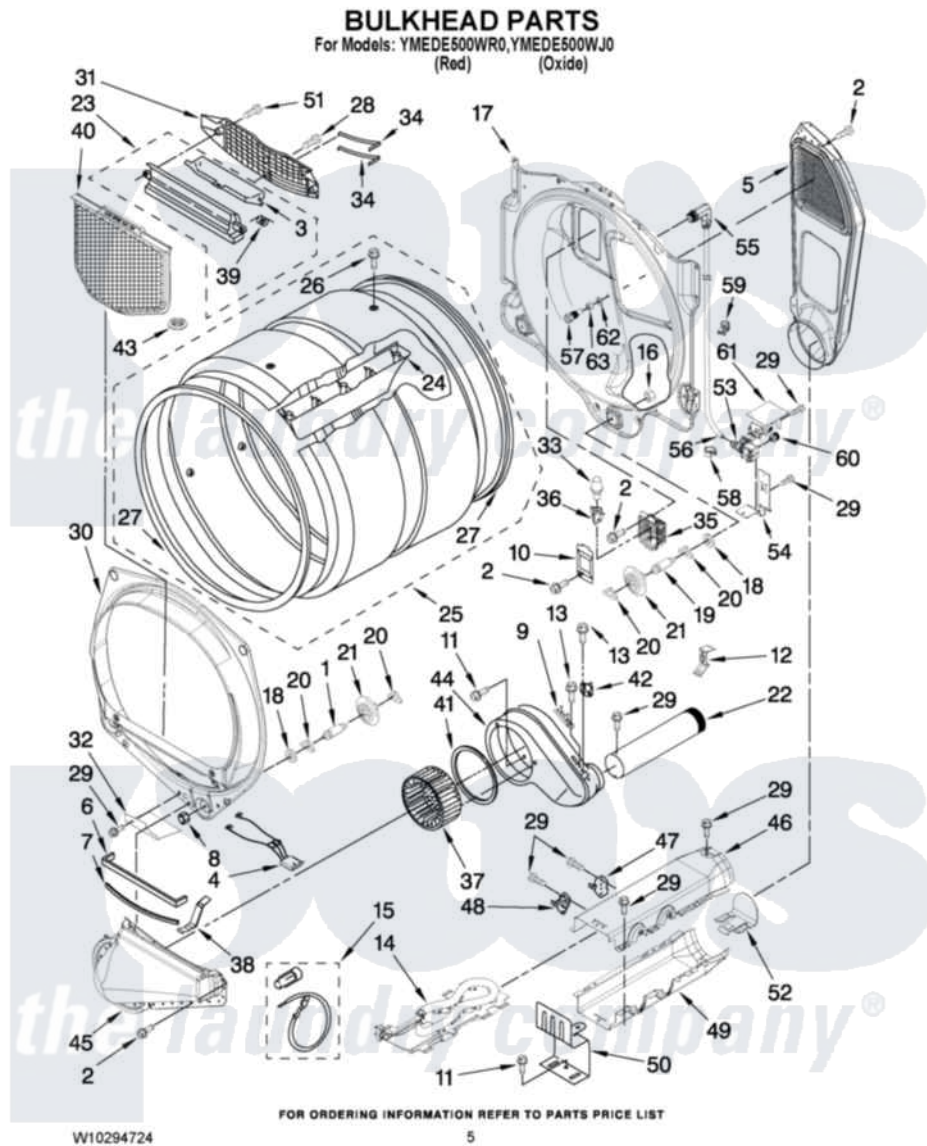
Maytag Residential Maytag YMEDE500WR0 Dryer Parts Parts Diagram 03 - BULKHEAD PARTS Click on the part number to view part
