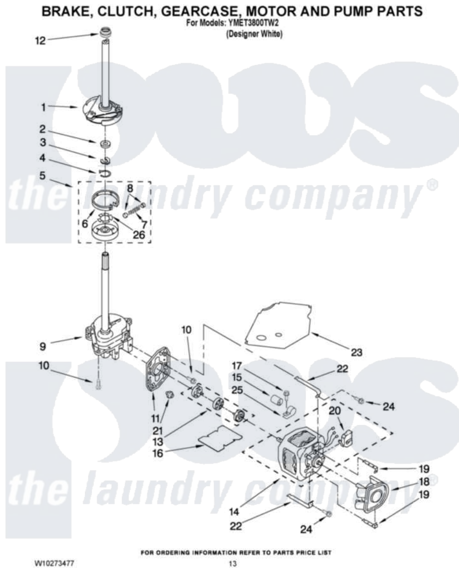
Maytag Residential Maytag YMET3800TW2 Washer/Dryer Parts Parts Diagram 08 - BRAKE, CLUTCH, GEARCASE, MOTOR AND PUMP PARTS Click on the part number to view part
