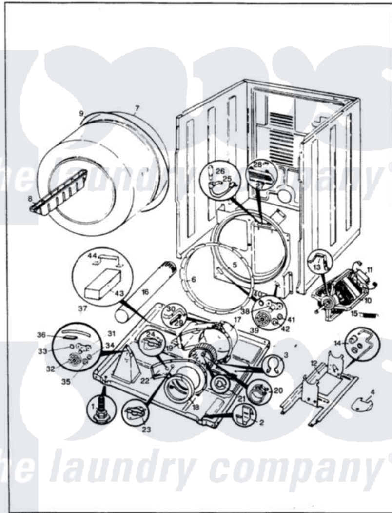
Norge Residential Norge DEL203W Dryer Parts Parts Diagram 03 - CYLINDER & DRIVE (REV. A-D) Click on the part number to view part
