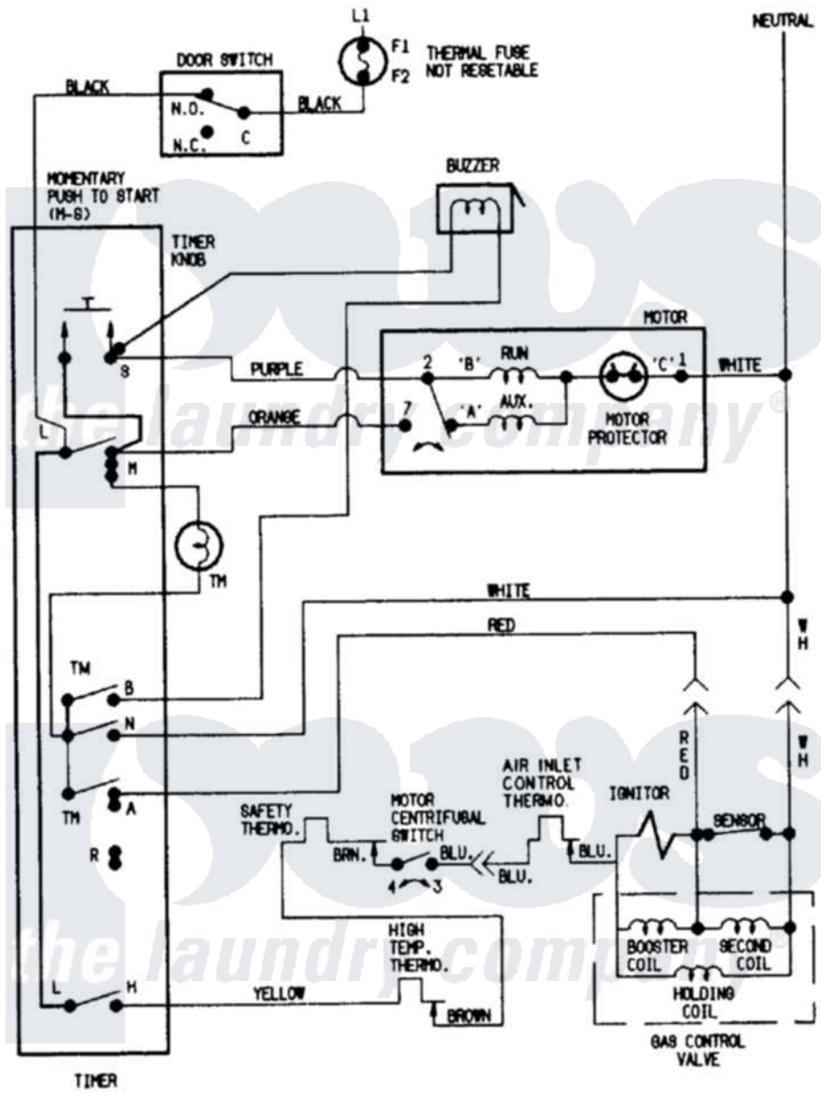
Norge Residential Norge DGN202W Dryer Parts Parts Diagram 07 - WIRING INFORMATION Click on the part number to view part
