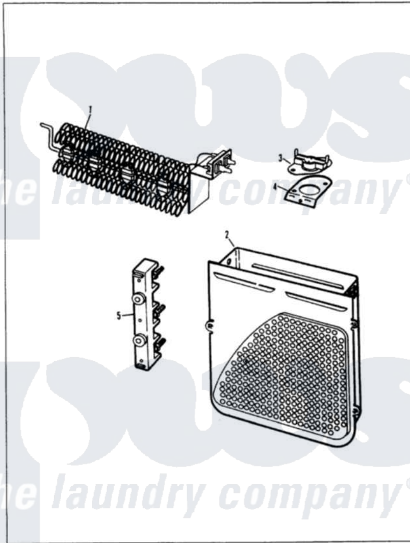
Norge Residential Norge LDE9127W Dryer Parts Parts Diagram 04 - HEATER Click on the part number to view part
