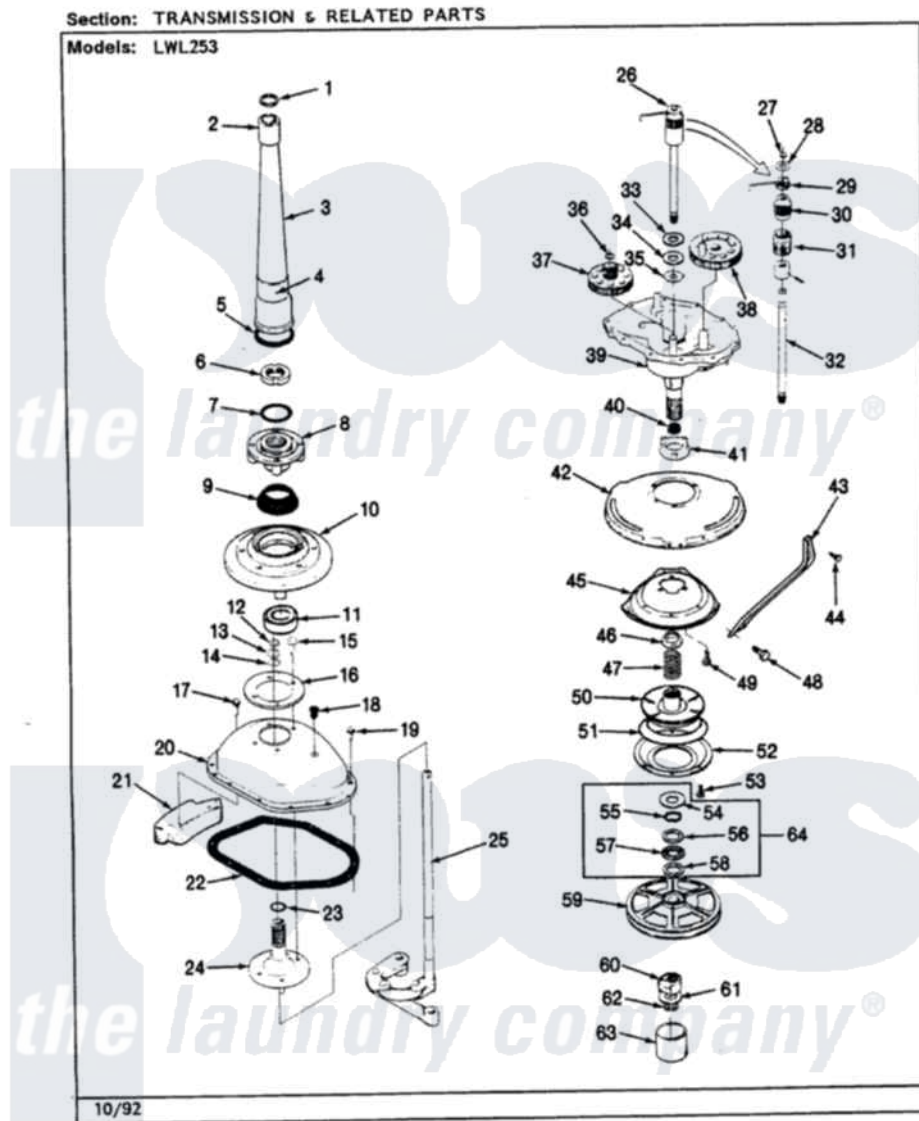
Norge Residential Norge LWL253A Washer Parts Parts Diagram 08 - TRANSMISSION & RELATED PARTS (REV. G-L) Click on the part number to view part
