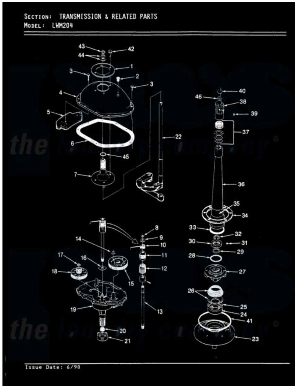
Norge Residential Norge LWM204A Washer Parts Parts Diagram 11 - TRANSMISSION & RELATED PARTS (REV. A-D) Click on the part number to view part
