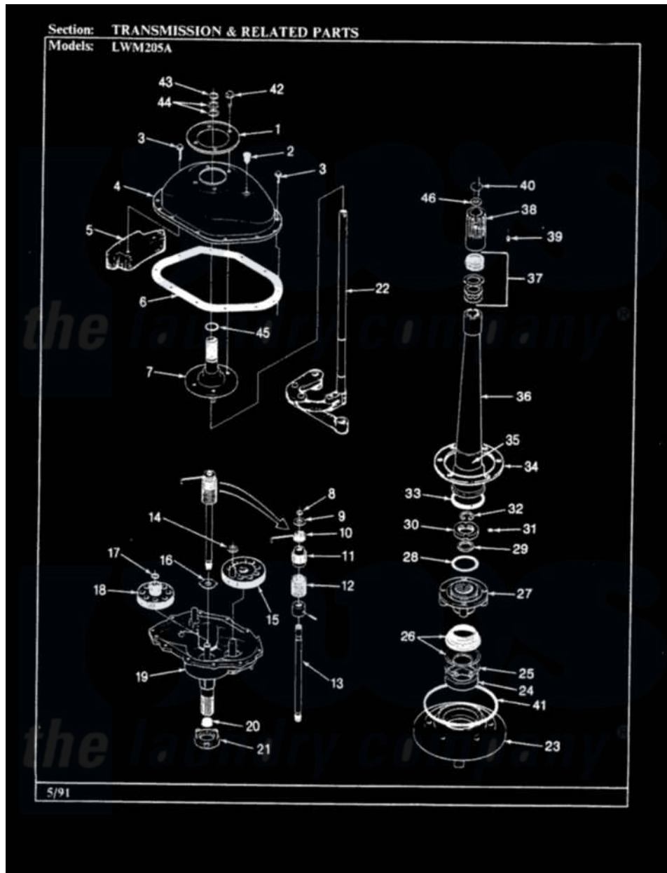
Norge Residential Norge LWM205A Washer Parts Parts Diagram 04 - TRANSMISSION & RELATED PARTS (ALM) Click on the part number to view part
