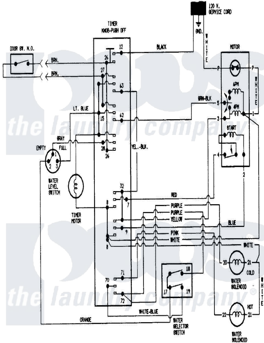
Norge Residential Norge LWN202W Washer Parts Parts Diagram 07 - WIRING INFORMATION Click on the part number to view part
