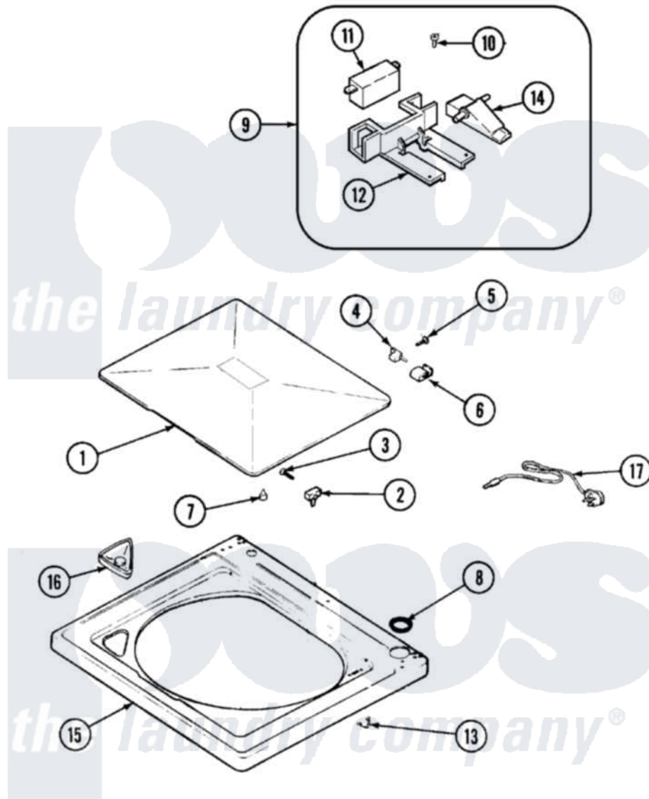
Norge Residential Norge LWP222V Washer Parts Parts Diagram 04 - TOP Click on the part number to view part
