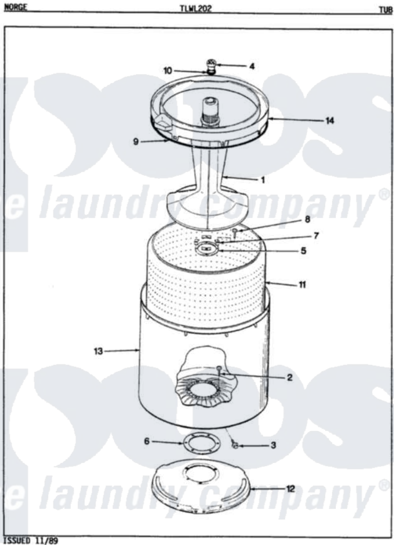
Norge Residential Norge TLWL202W Washer Parts Parts Diagram 05 - TUB Click on the part number to view part
