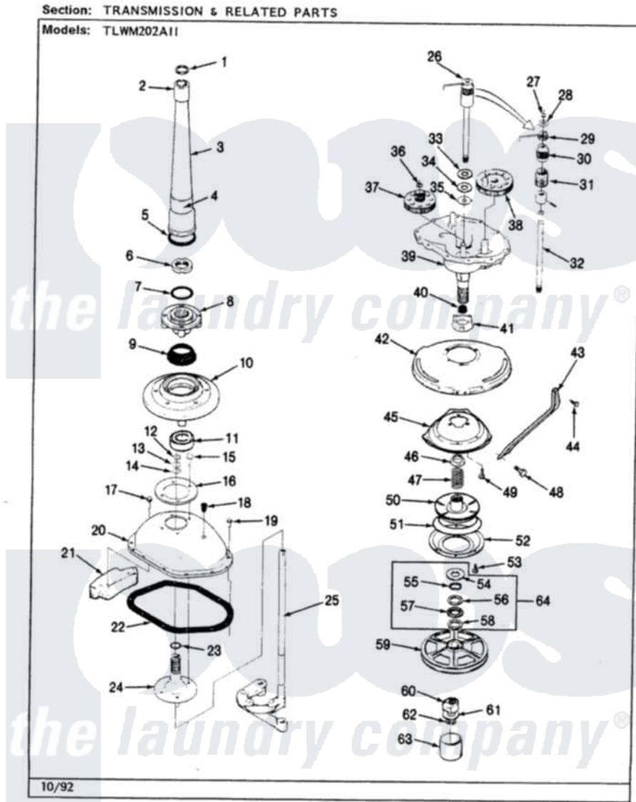
Norge Residential Norge TLWM202IIA Washer Parts Parts Diagram 07 - TRANSMISSION & RELATED PARTS (REV. F-K)
