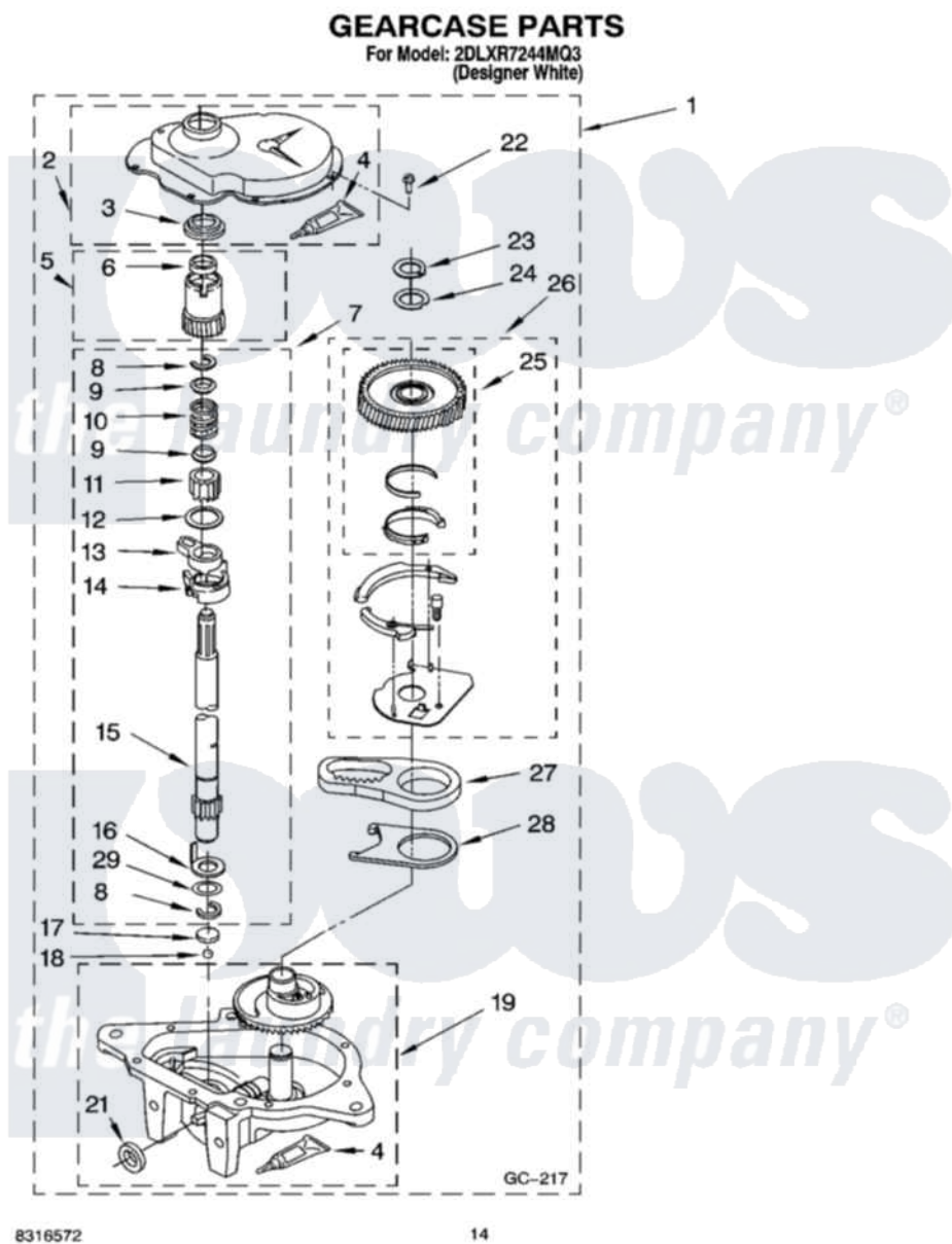
Whirlpool Residential Whirlpool 2DLXR7244MQ3 Washer Parts Parts Diagram 09 - GEARCASE PARTS, OPTIONAL PARTS (NOT INCLUDED) Click on the part number to view part
