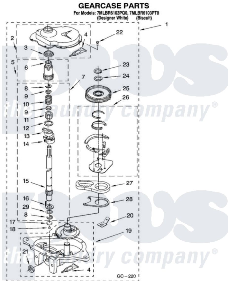
Whirlpool Residential Whirlpool 7MLBR6103PQ0 Washer Parts Parts Diagram 08 - GEARCASE PARTS Click on the part number to view part
