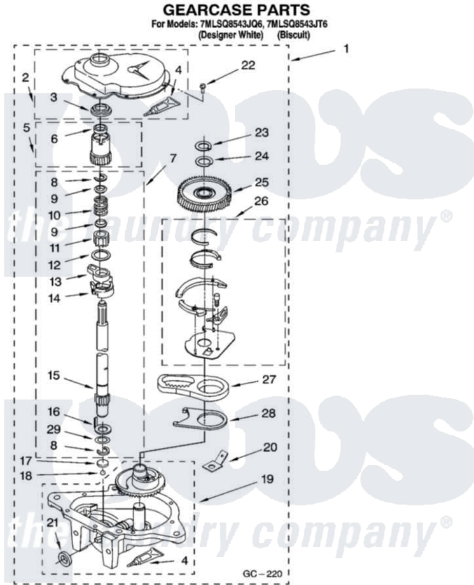
Whirlpool Residential Whirlpool 7MLSQ8543JQ6 Washer Parts Parts Diagram 08 - GEARCASE PARTS Click on the part number to view part
