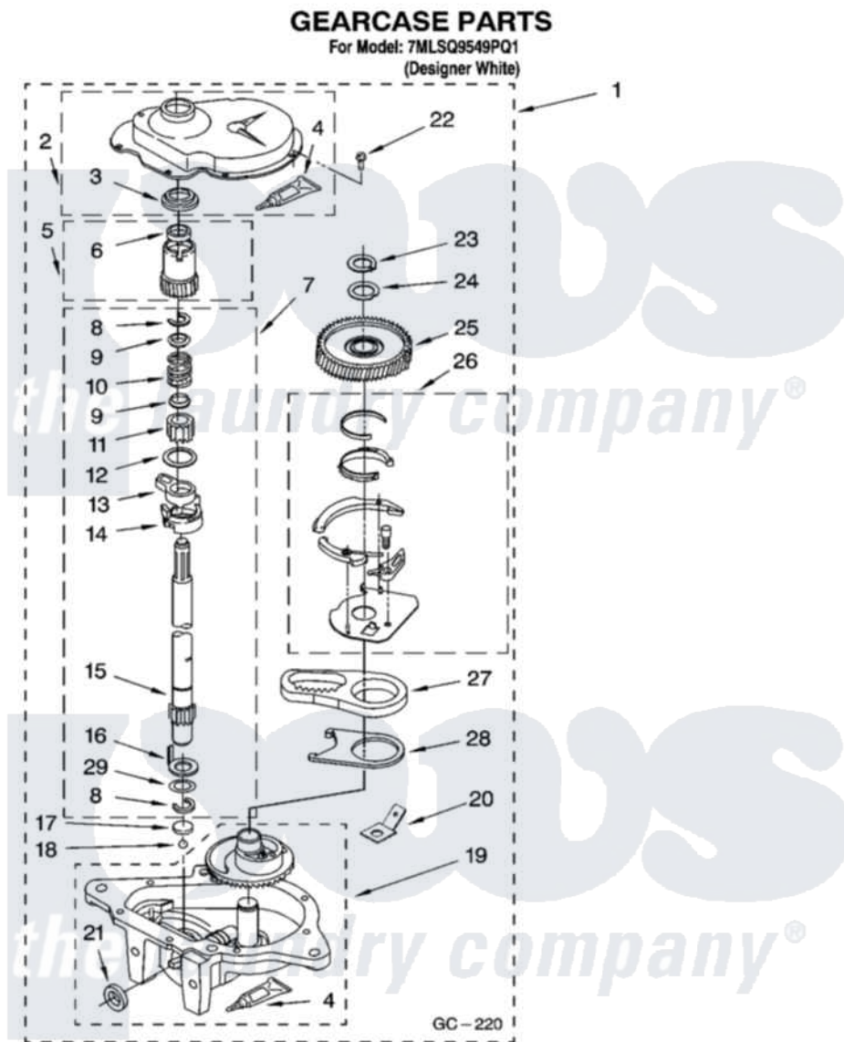
Whirlpool Residential Whirlpool 7MLSQ9549PQ1 Washer Parts Parts Diagram 08 - GEARCASE PARTS Click on the part number to view part
