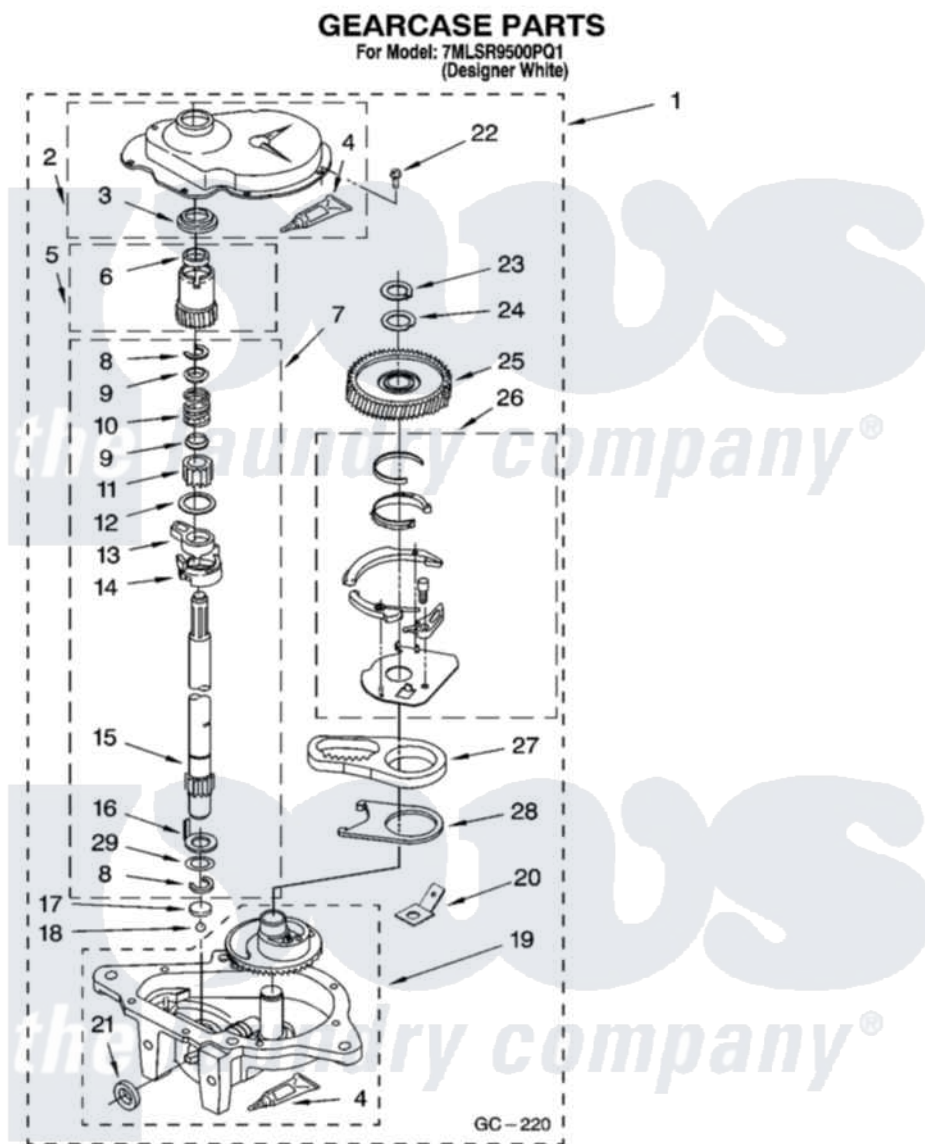
Whirlpool Residential Whirlpool 7MLSR9500PQ1 Washer Parts Parts Diagram 08 - GEARCASE PARTS Click on the part number to view part
