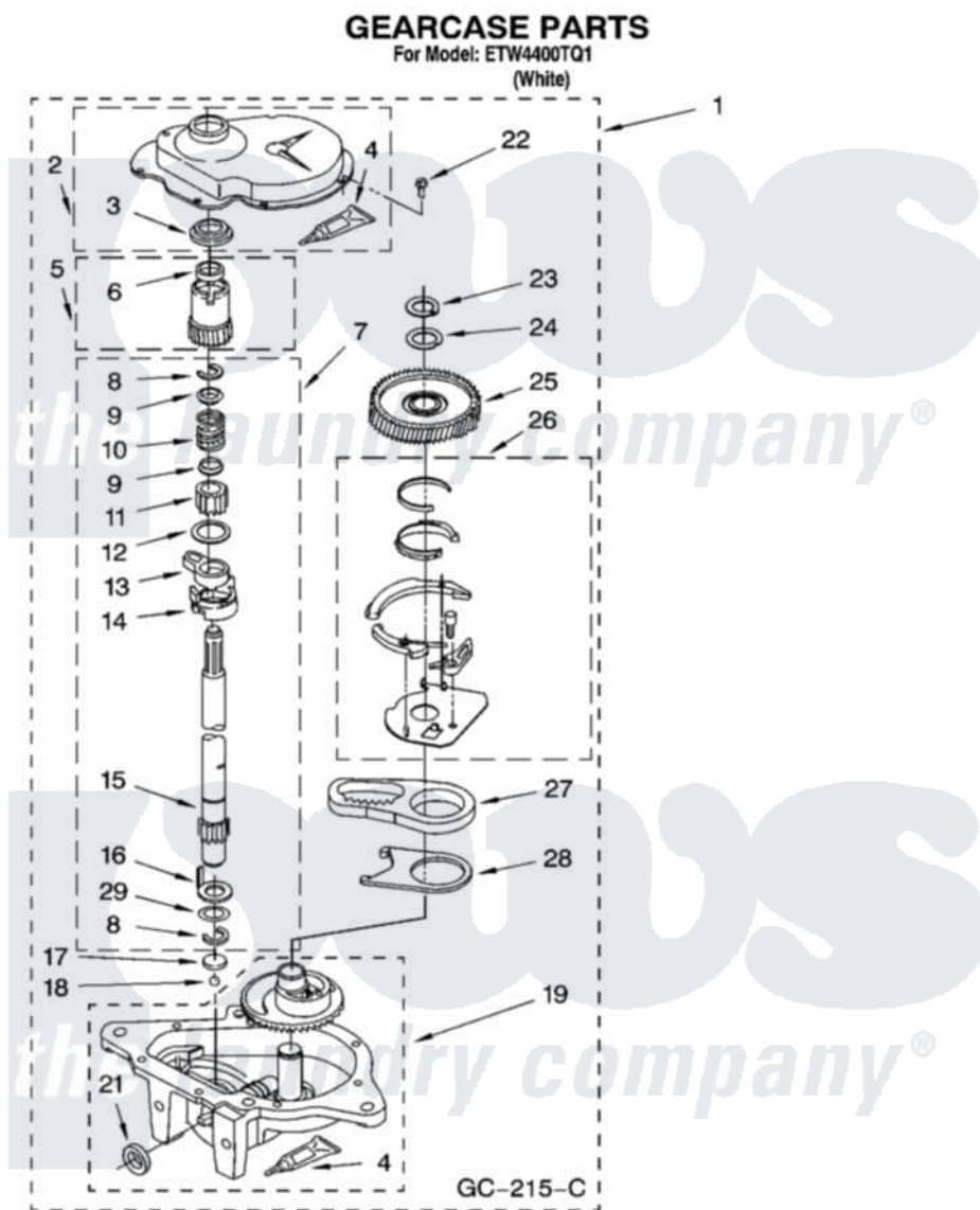
Whirlpool Residential Whirlpool ETW4400TQ1 Washer Parts Parts Diagram 08 - GEARCASE PARTS, OPTIONAL PARTS (NOT INCLUDED)
